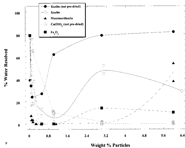
Figure 9. Effect of concentrations of various particles on water-in-crude oil emulsion stability.
