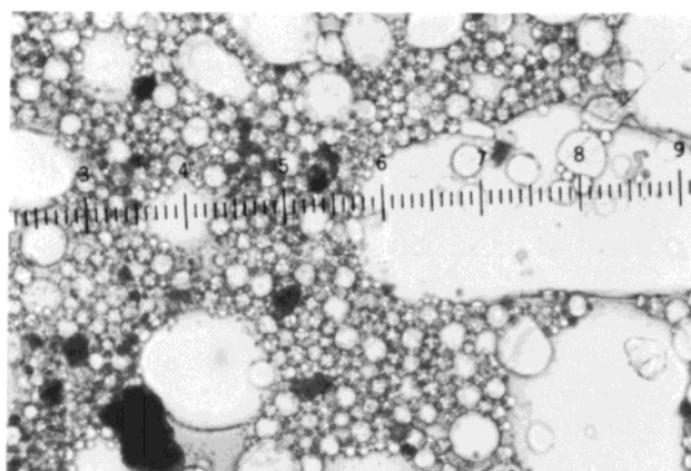
b. 0.5 % \text{Fe}_2\text{O}_3
